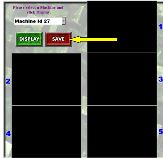
Figure 11 – Game Log
