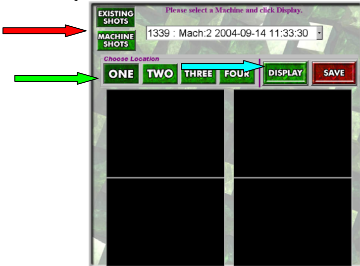
Figure 10 – Screen Shots
